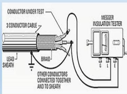
Insulation Resistance Test
